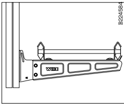
Cable ladder KHZSP mounted on Cantilever arm 50i, Profile clamp 42 is used.
