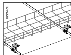
Mesh tray mounted across the seams of the roofing sheets with Combi bracket 53 and accessories from the Mesh tray programme.
