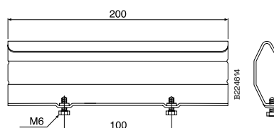
Joint 21 in stainless steel
