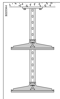
Mount Support bracket 3 on Vertical piece 20F with Screw set 2S.
