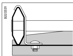
For installation of KHZSP, KHZ, KHZPV and KHZPS on Support bracket 3 Profile clamp 42 is used.
