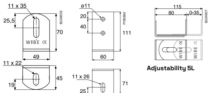
Angle bracket 5L
