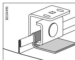
In order to avoid contact between Combi bracket 53 and copper sheeting, Insulating plate 54 must be used.
