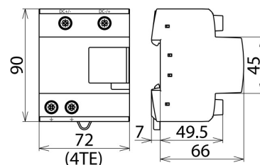
Dimensions DCB YPV 1500
