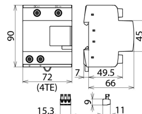
Dimensions DCB YPV SCI 1500 FM
