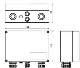
Dimensions DCU 2 YPV 1100 2M 1S
