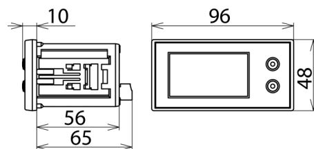
Dimensions DPAN L
