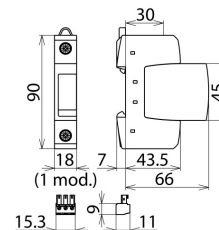
Dimensions DG S 150 FM
