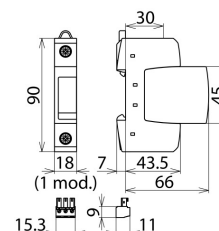
Dimensions DG S 385 FM
