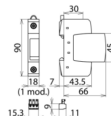
Dimensions DG S 600 FM
