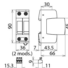
Dimensions DG M TN 275 FM
