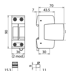
Dimensions DG M TN ACI 275 FM
