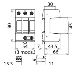
Dimensions DG M TNC 150 FM
