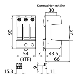
Dimensions DG M YPV SCI 1200 FM
