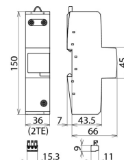
Dimensions DGPM 1 255 FM
