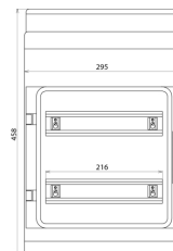
Dimension drawing IGA 24 IP54
