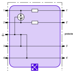
Basic circuit diagram BXT ML2 B 180
