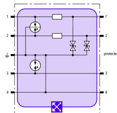
Basic circuit diagram BXT ML2 BE S 12
