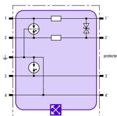
Basic circuit diagram BXT ML2 BD S 15
