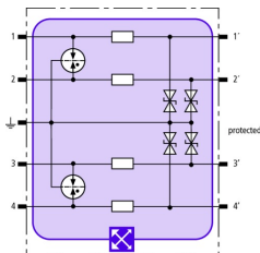
Basic circuit diagram BXT ML4 BE 180
