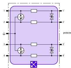
Basic circuit diagram BXT ML4 BD 180
