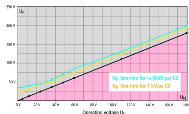
Diagram of the voltage protection level BXTU
