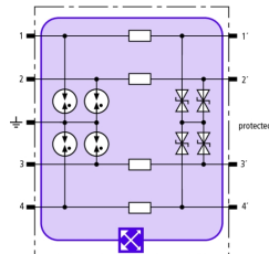
Basic circuit diagram BXT ML4 BC EX 24
