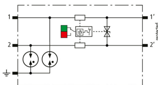
Basic circuit diagram BCO MOD ML2 BD 24
