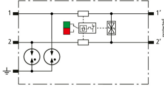
Basic circuit diagram BCO MOD ML2 BD HF 5
