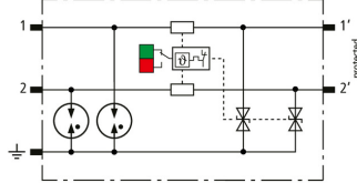
Basic circuit drawing BCO ML2 BE 24
