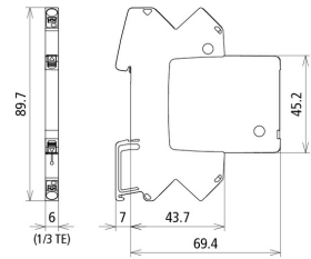
Dimension drawing BCO ML2 BE 24
