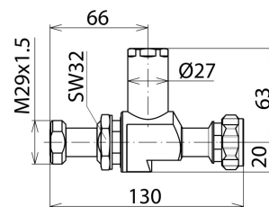
Dimension drawing DGA L4 7 16 MFA
