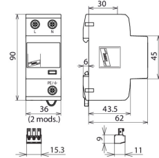
Dimension drawing DSH TN 255 FM
