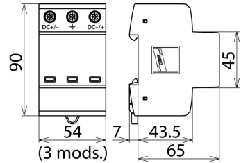
Dimension drawing DG YPV SCI 1000
