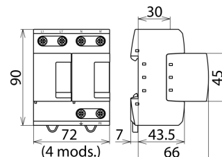
Dimension drawing DV M TT 2P 255
