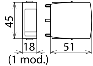
Dimension drawing DG MOD 150
