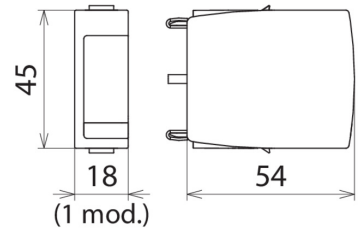
Dimension drawing DG MOD ACI 275
