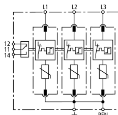
Basic circuit diagram DG M TNC 150 FM
