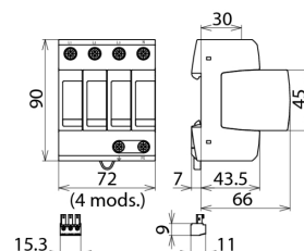
Dimension drawing DG M TNS 385 FM
