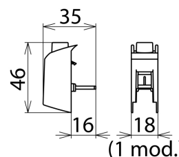
Dimension drawing STAK 25
