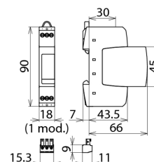
Dimension drawing DR M 2P 30 FM
