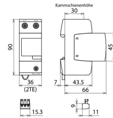
Dimension drawing DV M2 TN 255 FM
