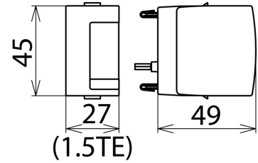
Dimension drawing DG MOD E DC 242
