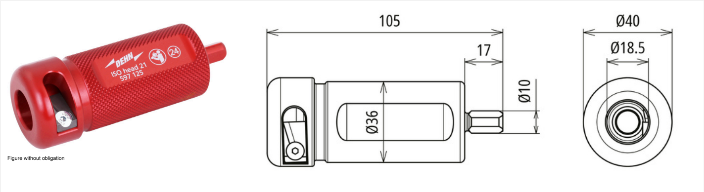
Cutting head for HVI light plus Conductor.
