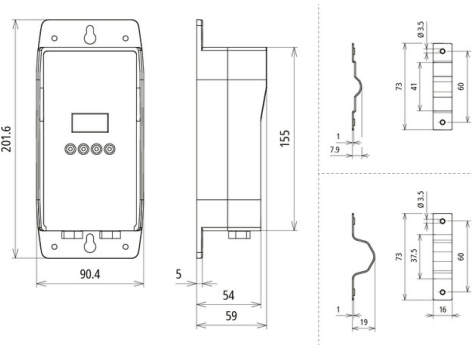
Dimension drawing DLSC 100
