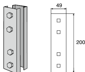
Pendelkoppeling 20J
