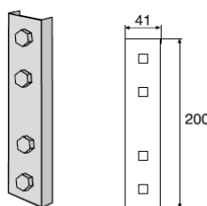
Pendelkoppeling 2J
