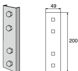
Pendelkoppeling 2FJ
