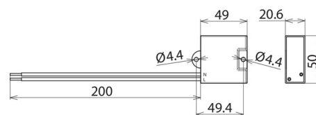
Dimensions DCOR L 1P 275
