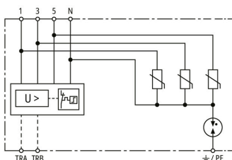
Basic circuit diagram POP+SPD 3P+N
