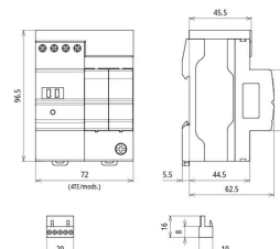
Dimension drawing POP+SPD 3P+N
