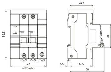
Dimension drawing POP+RU+MCB+SPD 25A 1P+N
