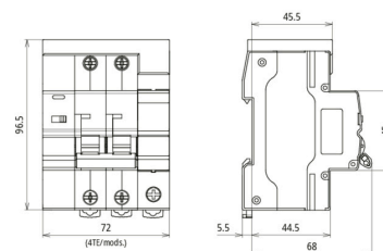
Dimension drawing POP+RU+MCB+SPD 40A 1P+N
