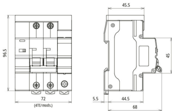
Dimension drawing POP+RU+MCB+SPD 50A 1P+N
