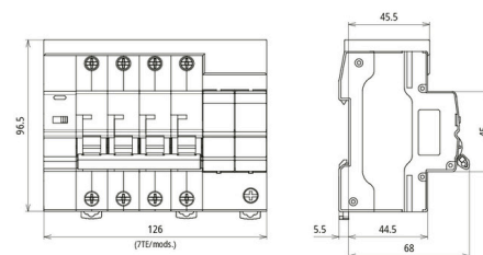
Dimension drawing POP+RU+MCB+SPD 63A 3P+N
