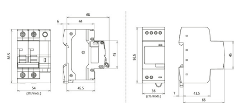
Dimension drawing SPD+POP+MCB 25A 1P+N T1+2
