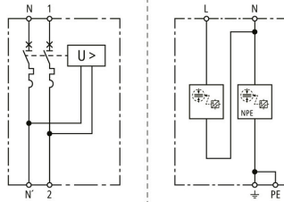
Basic circuit diagram SPD+POP+MCB 32A 1P+N T1+2
