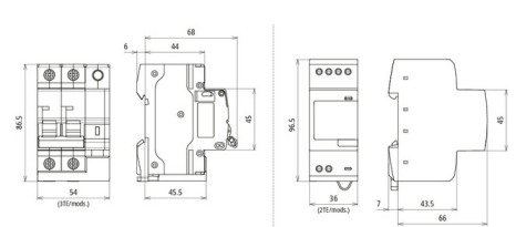
Dimension drawing SPD+POP+MCB 32A 1P+N T1+2
