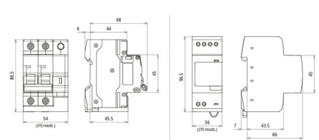
Dimension drawing SPD+POP+MCB 40A 1P+N T1+2
