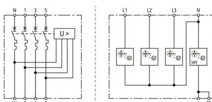
Basic circuit diagram SPD+POP+MCB 32A 3P+N T1+2
