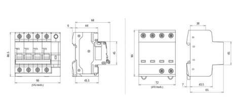
Dimension drawing SPD+POP+MCB 63A 3P+N T1+2
