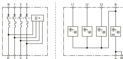
Basic circuit diagram SPD+POP+MCB 63A 3P+N T1+2
